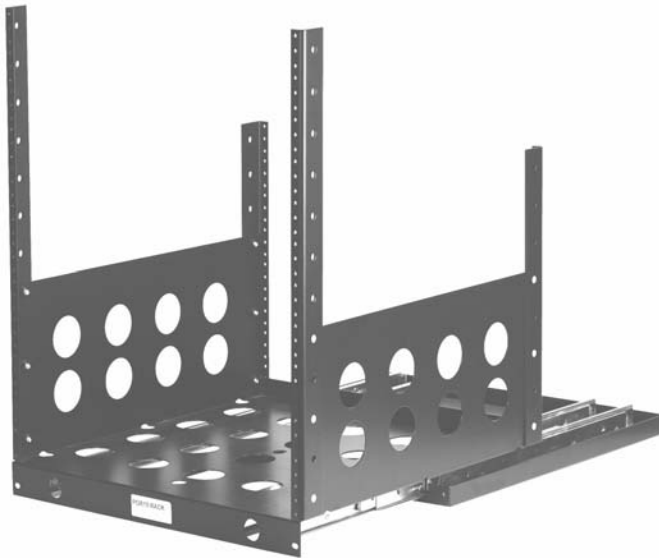
POR194-10 Shown partially extended.
