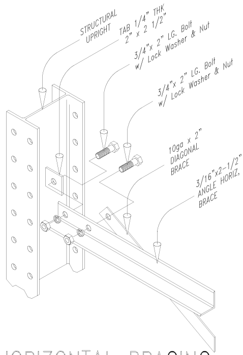
HORIZONTAL BRACING AND X-BRACING INSTALLATION
